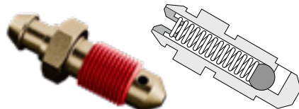
Speed Bleeder
